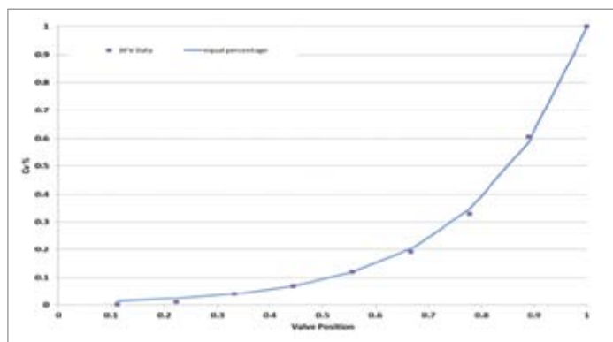
Figure 2: Butterfly Valve C_v Curve
