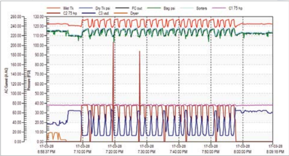
Figure 3: A control gap problem shows the air compressor fighting for lead control.
